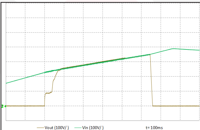
Figure 11: Turn-on and Turn-off behavior as a function of V_{in} . ENA previously enabled. Ch 1: V_{out} (100 V/div). Ch 2: V_{in} (100 V/div). Timescale: 100 ms/div.
