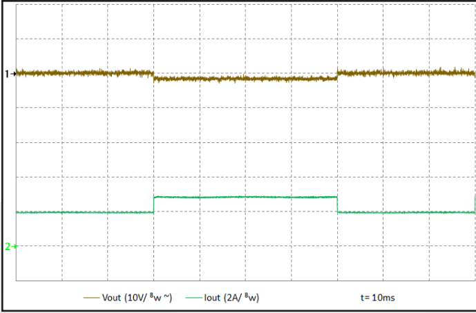
Figure 13: Output voltage response to step-change in load current 50%-75%-50% of I_{out} (max). Zero output capacitance. Ch1: V_{out} (10 V/div). Ch 2: I_{out} (2 A/div). Timescale: 10 ms/div. Plot created using measured V_{out} minus V_{in} / Turns Ratio.
