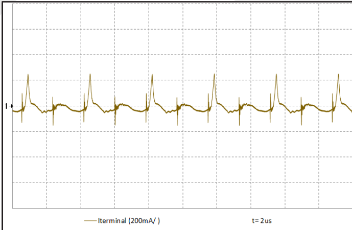
Figure 15: Input terminal ripple, i_c , at full load and nominal voltage with 10 \mu H source impedance and 100 \mu F electrolytic capacitor(200 mA/div), Bandwidth: Full. Timescale: 2 \mu s/div. See Figure 12.
