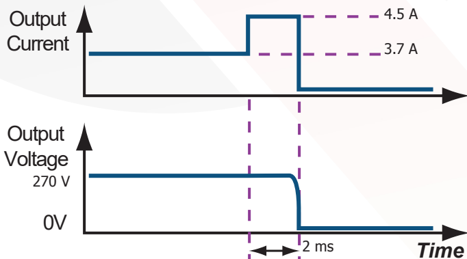
Figure D: Output Overload protection diagram (not to scale)
