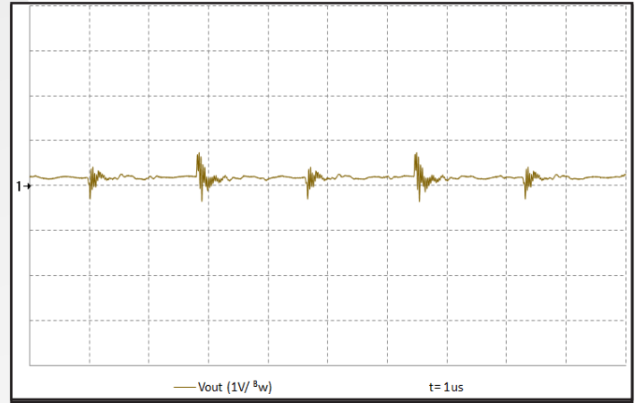
Figure 16: Output voltage ripple, V_{out} , at nominal input voltage and full load (1 V/div), Measured with 1.1 \mu F capacitance across the output terminals. Bandwidth: 20 MHz. Timescale: 1 \mu s/div. See Figure 12.
