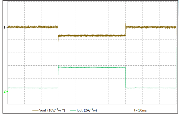
Figure 14: Output voltage response to step-change in load current 10%-100%-10% of I_{out} (max). Zero output capacitance. Ch1: V_{out} (10 V/div). Ch 2: I_{out} (2 A/div). Timescale: 10 ms/div. Plot created using measured V_{out} minus V_{in} / Turns Ratio.
