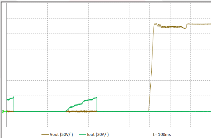
Figure 17: Rise of output voltage after the removal of a short circuit across the output terminals. R_{short} = 5 \text{ m}\Omega . Zero output capacitance. Ch1: V_{out} (50 V/div). Ch 2: I_{out} (20 A/div). Bandwidth: Full. Timescale: 100 ms/div.
