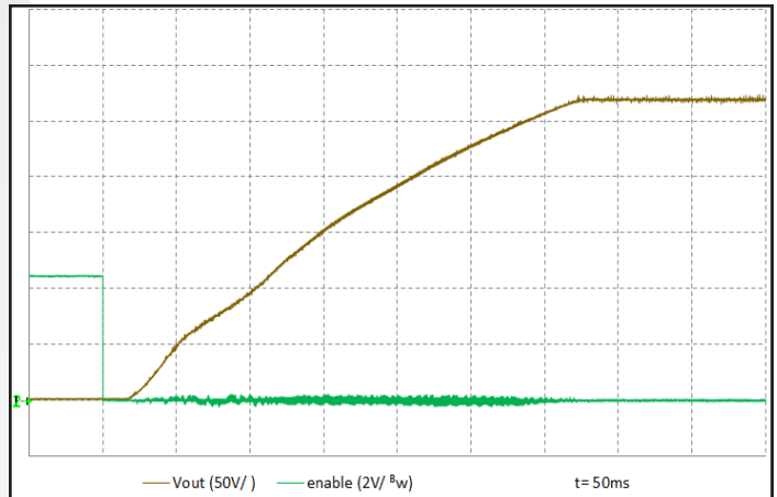
Figure 10: Turn-on transient at half resistive load and 400 \mu\text{F} output capacitance initiated by ENA. Input voltage pre-applied. Ch 1: V_{out} (50 V/div). Ch 2: ENA (2 V/div). Timescale: 50 ms/div.
