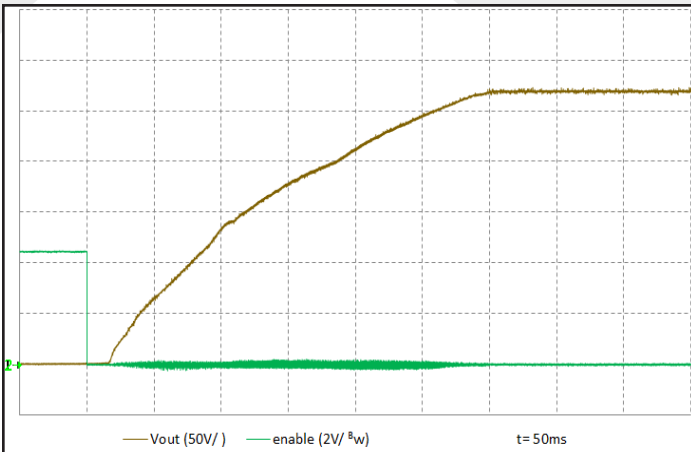
Figure 9: Turn-on transient at half resistive load and 47 \mu\text{F} output capacitance initiated by ENA. Input voltage pre-applied. Ch 1: V_{out} (50 V/div). Ch 2: ENA (2 V/div). Timescale: 50 ms/div.
