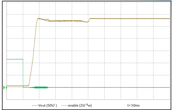
Figure 8: Turn-on transient at no load and zero output capacitance initiated by ENA. Input voltage pre-applied. Ch 1: V_{out} (50 V/div). Ch 2: ENA (2 V/div). Timescale: 50 ms/div.
